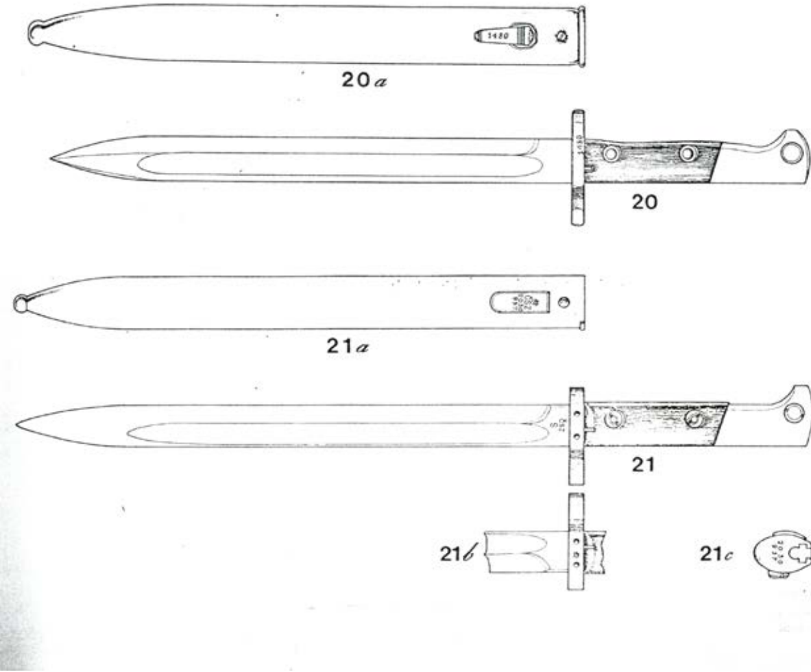
20) Bayonet for Uruguayan Mauser rifle Model 1908 Steel grip and crosspiece. Walnut scales. Total length 41.5 cms.
